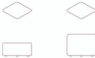
DIMENSIONS / CM: LEGO II-3: L 100 D 60 H 45 LEGO II-4: L 100 D 60 H 75
